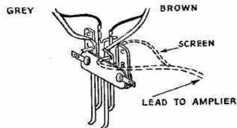
Connections for Monophonic Pickups Diagram Three
